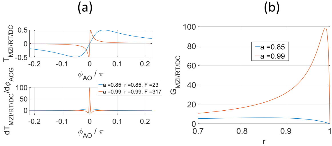
Figure 6.5 (a) MZI/RT/DC transfer function and its derivative as a function of phase. (b) G_{MZI/RT/DC} as a function of r for different value of a .
