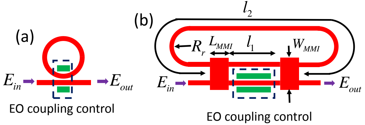
Figure 5.11 EO tuning of the coupling condition. (a) Ring resonator with gap based DC. (b) Proposed RT resonator with MZI based coupler consisting of two MMI couplers and two parallel waveguides.
