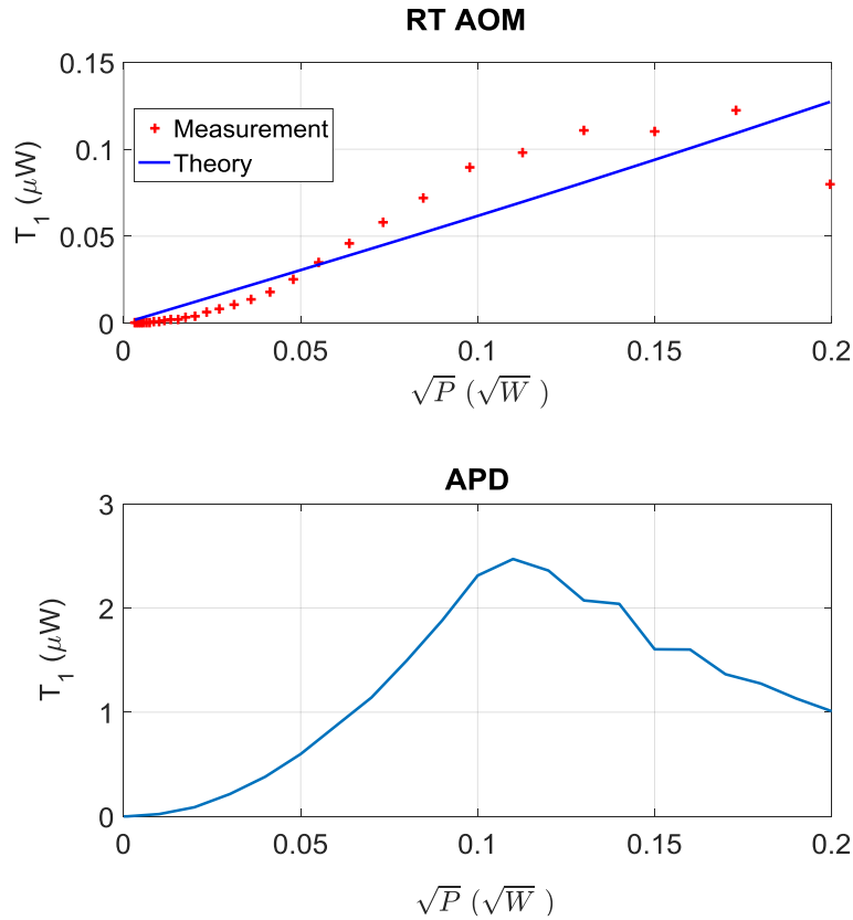
Figure 5.16 compares the measured modulation response with theory in the top sub-figure. The discrepancy between the theory and the measurements is attributed mostly to the non-linearity of the APD which is characterized separately in the bottom portion of the figure. Additionally, it might be attributed to the non-linearity in the transduction efficiency of the IDT at the low modulating power levels. Nonetheless, the results confirm that the value for the AO M_2 coefficient of the LN thin film is close to the expected theoretical value.
