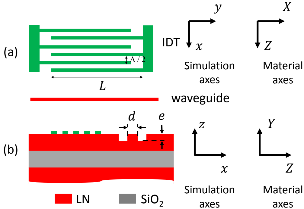
Figure 5.10 Waveguide placed near the IDT. The Capital letters (X, Y, and Z) denote the material axes while the small letters (x, y and z) denote the simulation axes. (a) Top view. (b) Side view.
