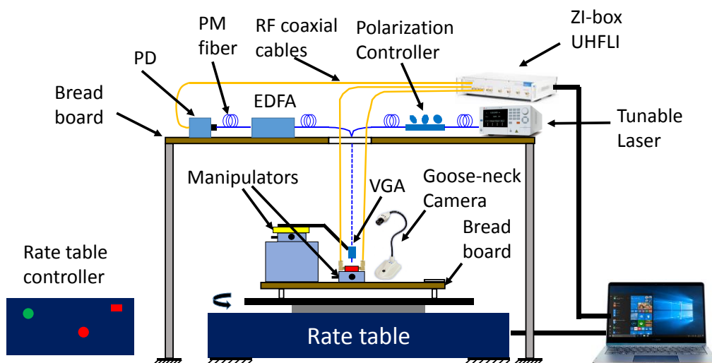
Figure 6.11 AOG measurement setup. The optical setup with the positioners and manipulators are mounted on top of the rate table.
