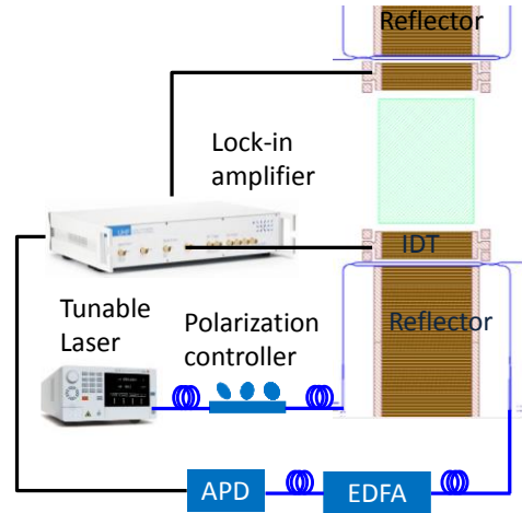
Figure 5.7 AOM measurement setup using lock-in amplifier.
