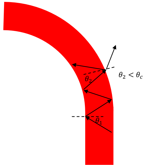
Figure 3.7 Ray picture describing the bending radiation loss
